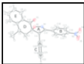
Fig. 1. The molecular structure of (I), showing the crystallographic atom-numbering scheme and displacement ellipsoids drawn at the 50% probability level.
