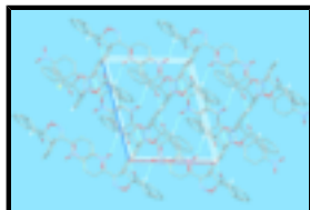
Fig. 2. The crystal packing of (I), viewed down the b axis. The C—H...O contacts are shown as dashed lines. H atoms not involved in C—H...O contacts have been omitted for clarity.
